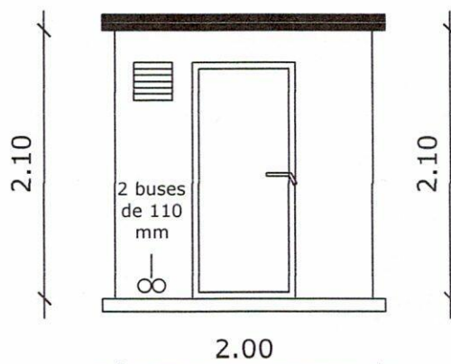
façade principale
